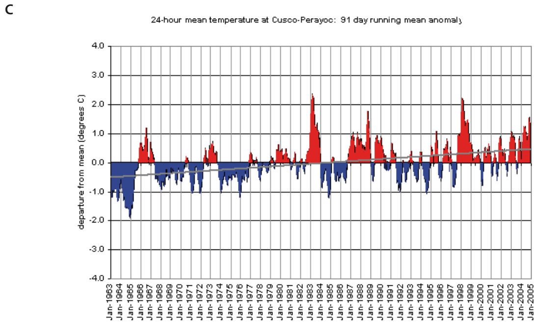
Figure 14. Long-term Temperature Record for (a) Minimum, (b) Maximum, and (c) Average Temperature in Cusco, Peru (continued)
